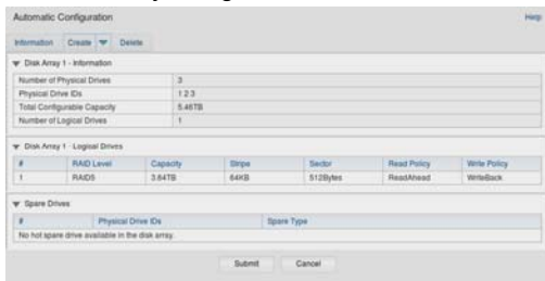
Figure 29: Automatic Disk Array Configuration menu
