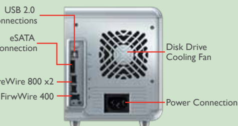
USB 2.0 Connections
