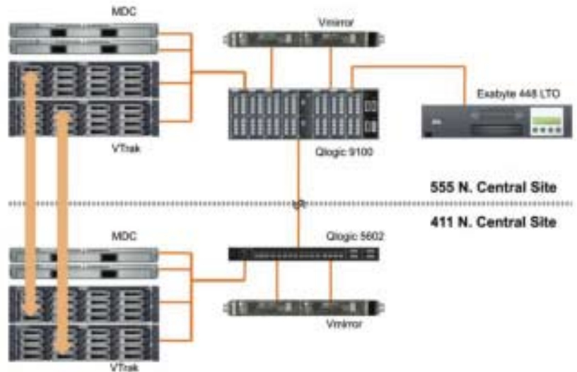
Figure 2. Cronkite School Play-to-Air SAN Configuration
